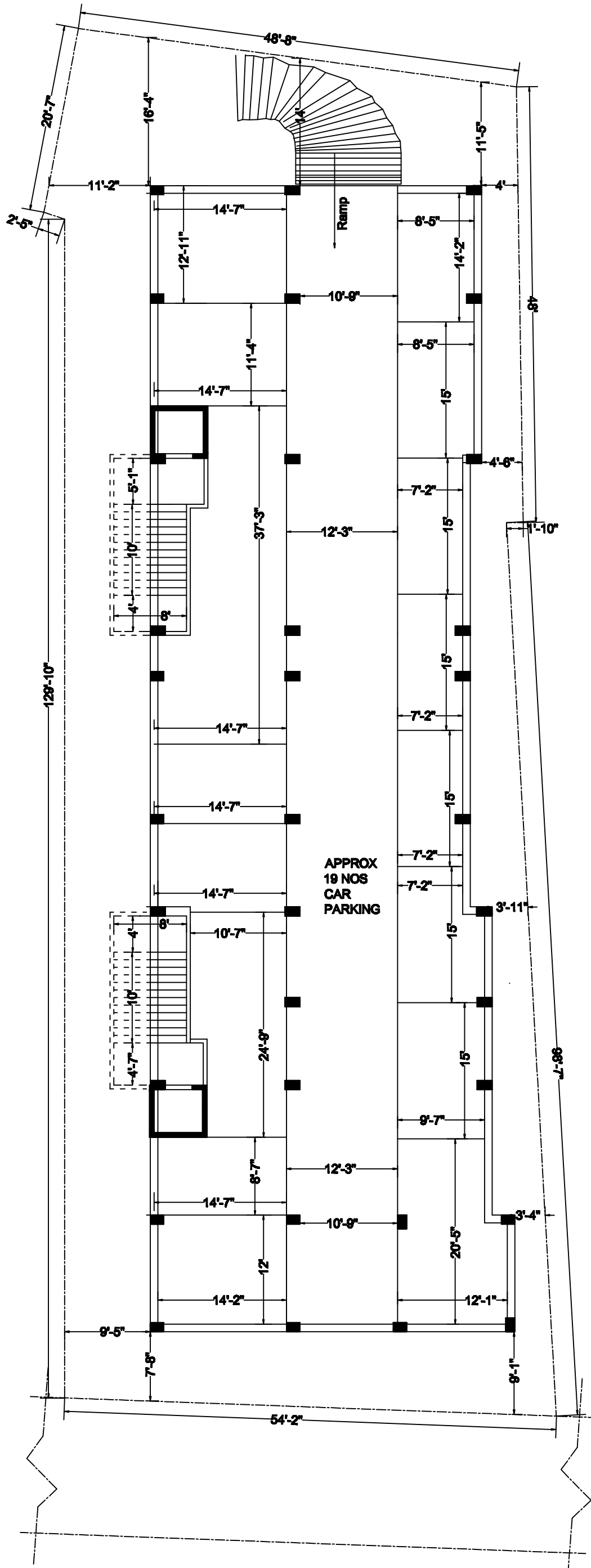
BASEMENT FLOOR PLAN SCALE-1"=8'-0" TOTAL . AREA = 4630 SFT.
